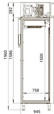
bokorys DM 114
