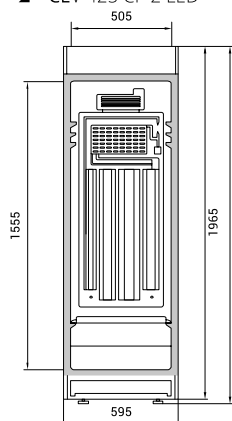
CEV 425 CP 2 LED
