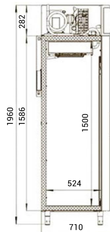
bokorys DM 110
